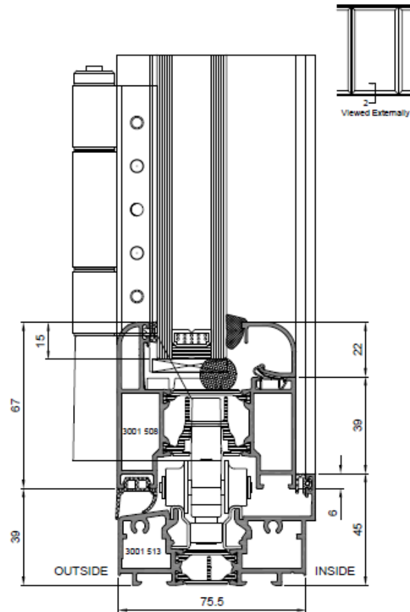
Standard threshold (with full weather rating)
