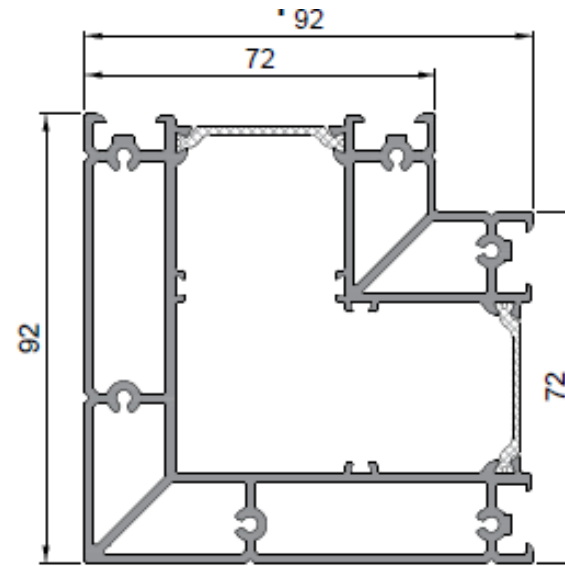
Corner post (option)
