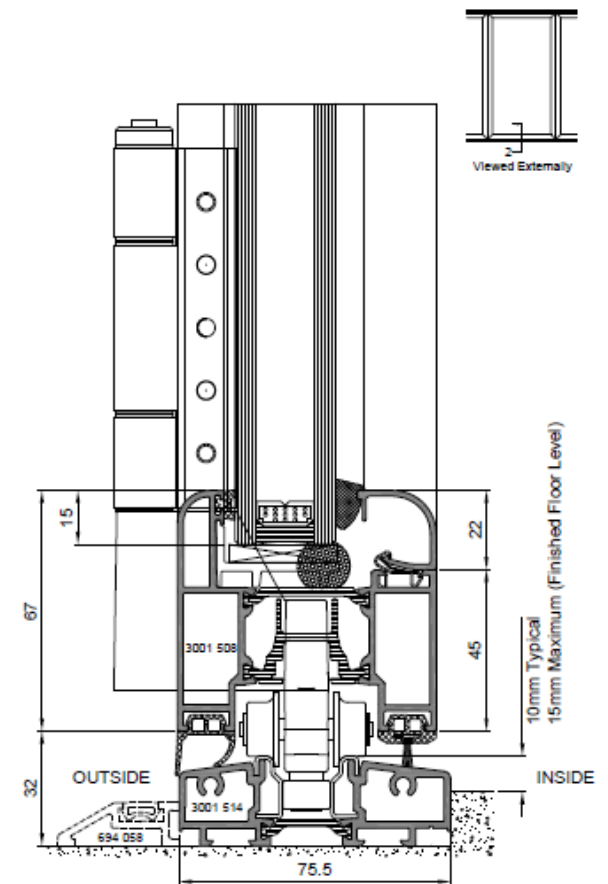
Low threshold (not severe weather rated)
