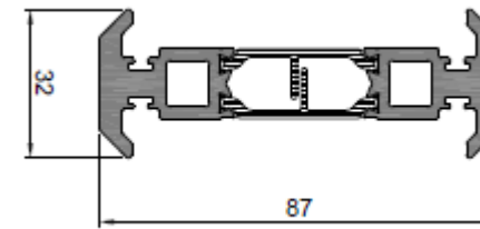
15mm coupler
