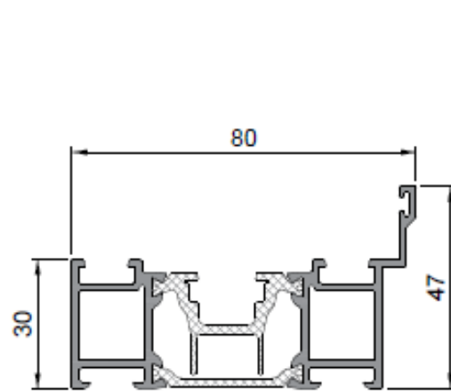
3001 512 Rebated head/jamb 6700mm stock length
