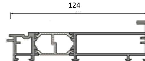
Sub cill detail – twin track
